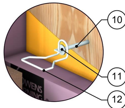
Anchor Detail
