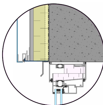
Head Detail
