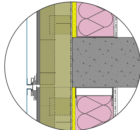
Intermediate Floor Detail
