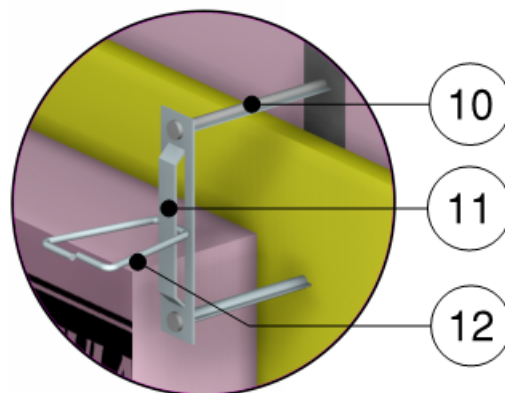
X-Seal Byna-Lok Anchor Detail
