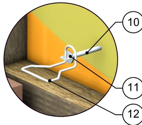
Anchor Detail
