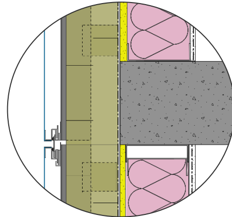
Intermediate Floor Detail
