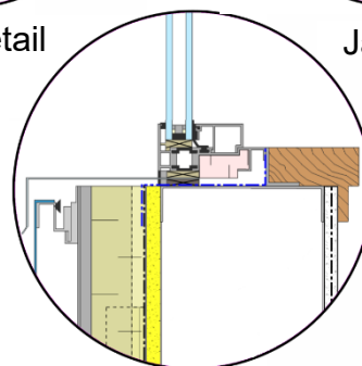
Sill Detail
